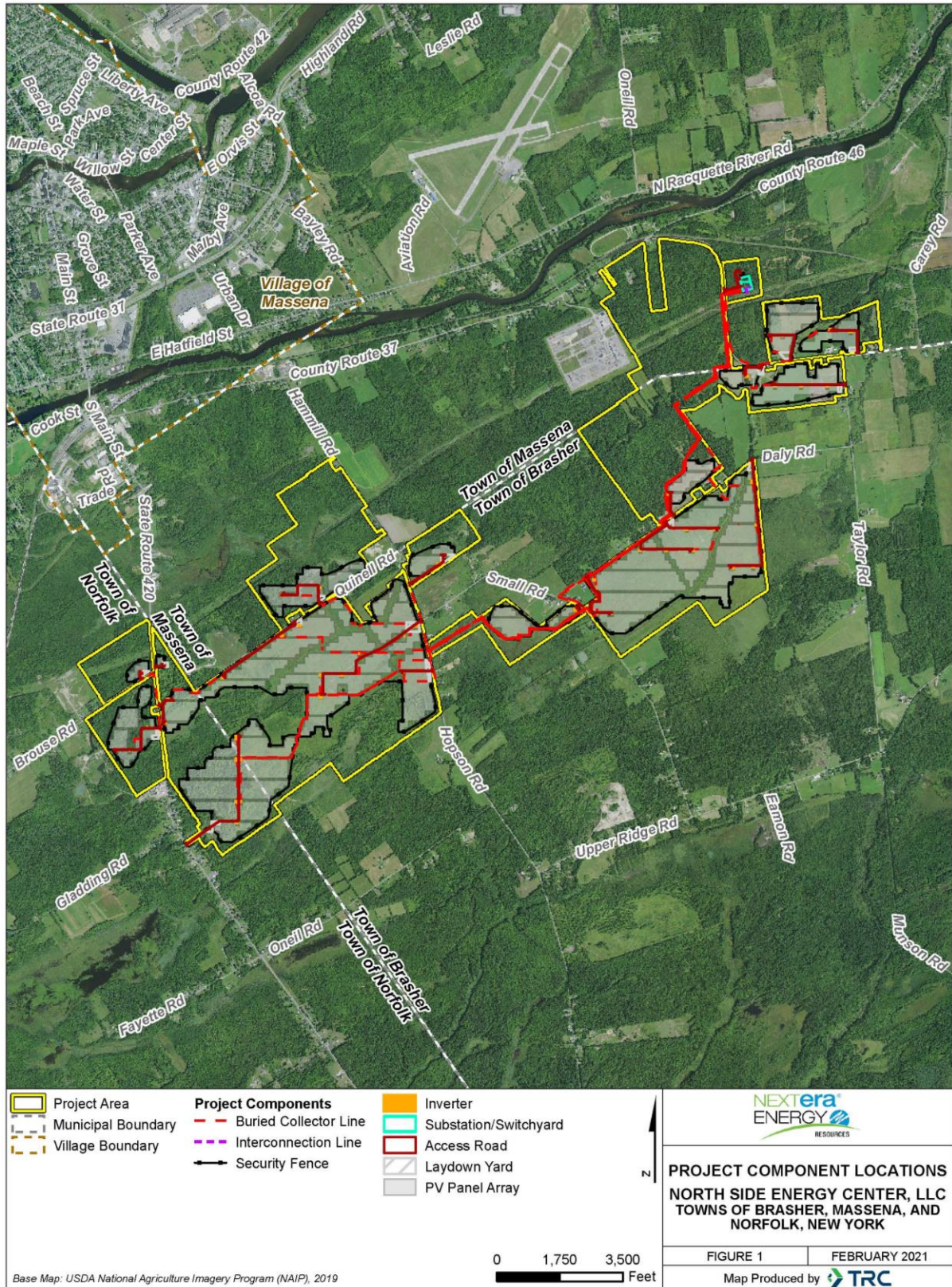
Figure 1. General Layout of North Side Energy Center
